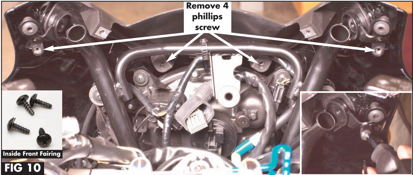
Fig 10. Remove all 4 phillips screw, located behind the inner fairing. See FIG10.
