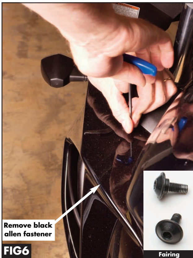
Fig 6. Remove 2 allen fastener closest to the tank. (For Both Sides) See FIG6. Note: The finish allen screws are in black.
