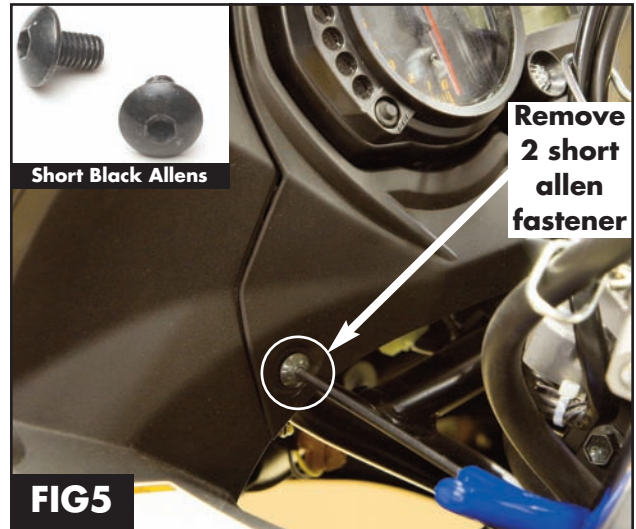
Fig 5. On the same plastic fairing, remove 2 black short allen fastener located on the bottom of the instrument cluster. (For Both Sides) See FIG5. Note: The finish allen screws are in Black.
