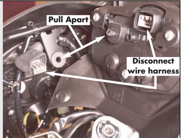
Fig 7. Remove instrument panel by pulling it apart from the fairing frame. The wire harness needs to be disconnected before fully removing. USE CAUTION TO NOT OVER PULL!!!
